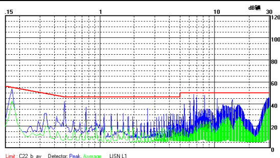
DEZ-0505-XT1P CE(Class B, Positive line)
