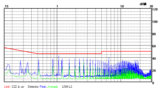
DEZ-1205-XT1P CE(Class B, Negative line)
