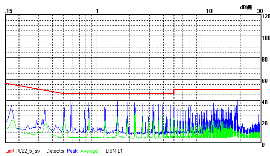
DEZ-1205-XT1P CE(Class B, Positive line)
