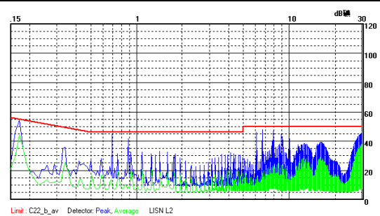
DEZ-0505-XT1P CE(Class B, Negative line)
